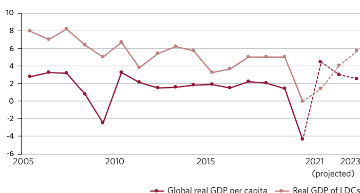
Annual growth rate of global real GDP per capita and annual growth rate of real GDP of LDCs, 2005–2023 (percentage)
