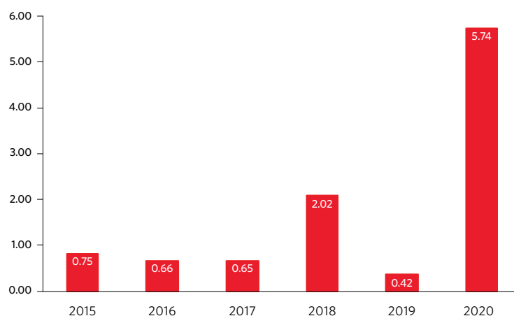
Disaster-related mortality (rate per 100,000 population), 2015-2020
