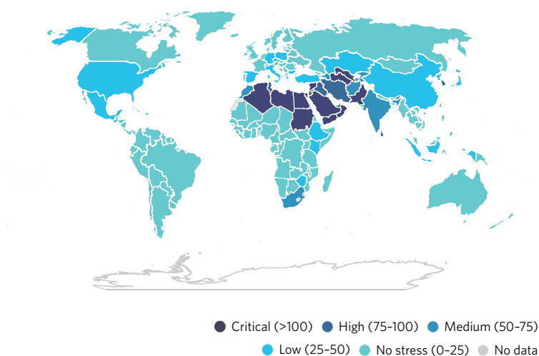
Level of water stress: freshwater withdrawal as a proportion of total renewable freshwater resources, 2019 (percentage)
